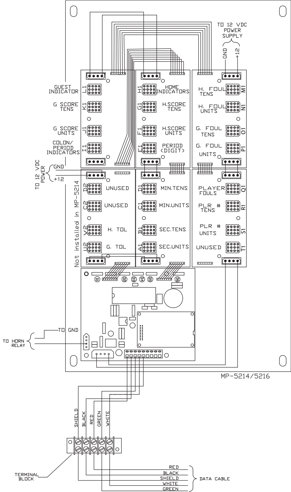
CONTROLLER WIRING
