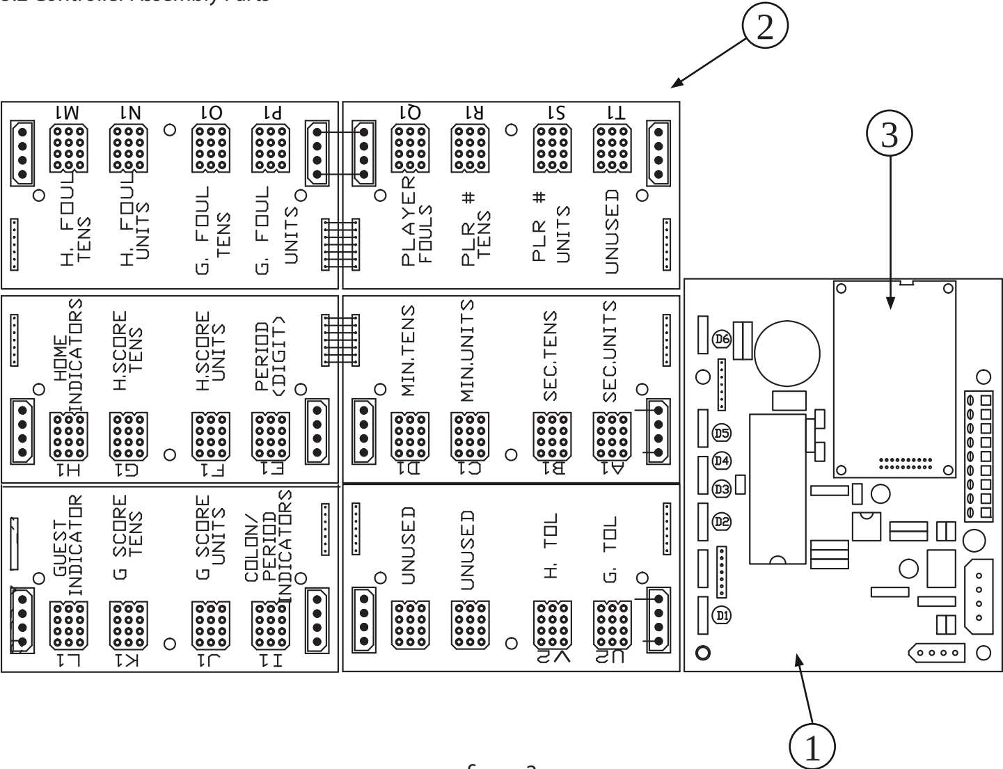
figure 2 CONTROLLER ASSEMBLY
